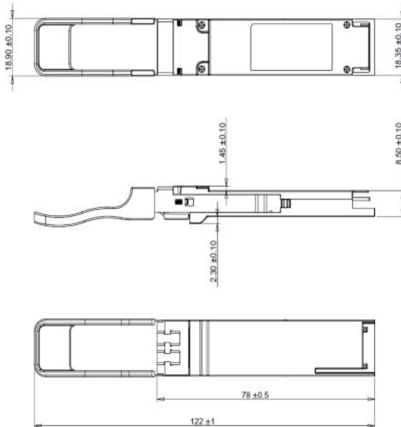
Figure 4. Mechanical Outline
