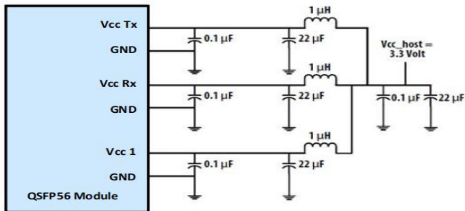
Figure 3. Recommended Power Supply Filter
