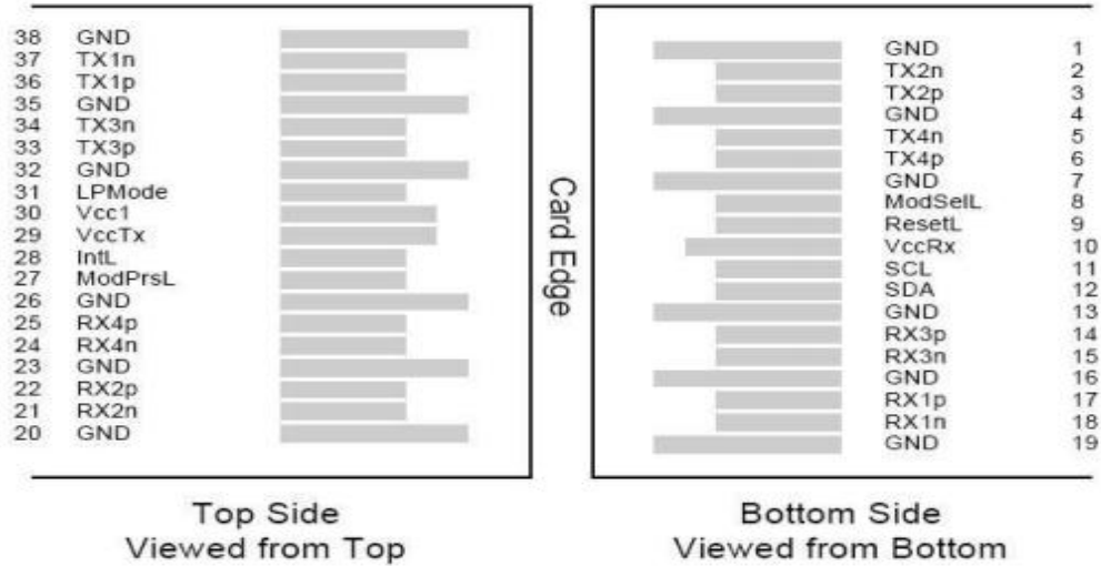
Figure 2. MSA Compliant Connector
